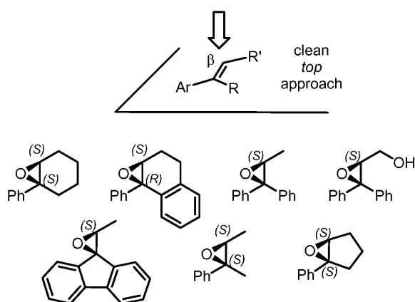
Figure 7. Facial selectivity.
